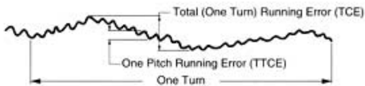
Fig. 15-3 Example of Dual Contact Running Testing Report
