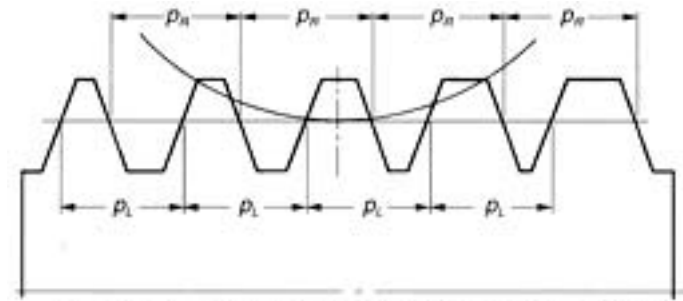
Fig. 14-12 Basic Concepts of Duplex Lead Worm
